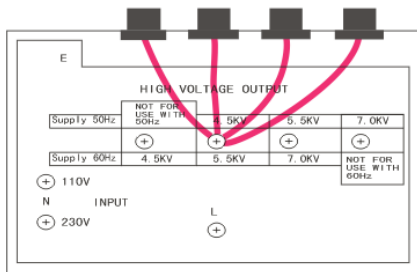
A, Connects 4x4. 5KV
